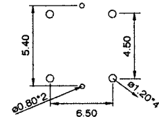
P.C. Mounting
